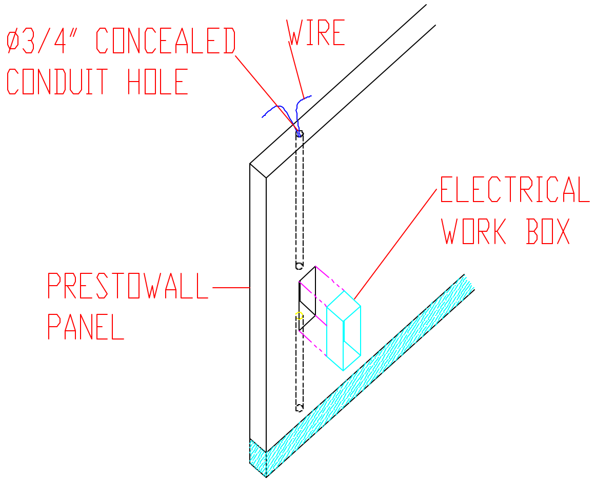
Electrical Box Details (Use Plunge router to clean out hole)
