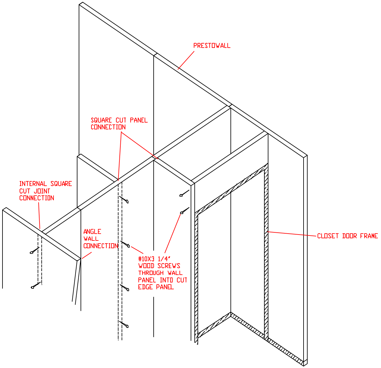
Internal Wall Layout
